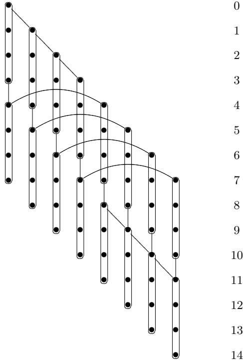
Figure 1. Proof of Theorem 1.2.
