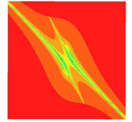
\kappa = 75, \lambda = 1.5
